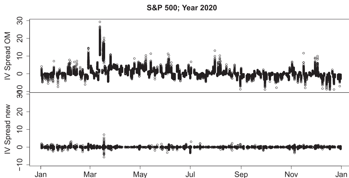
FIGURE 2 IV spreads of S&P 500 options in 2020. The IV spread is defined as the difference between the IVs of pairs of puts and calls (in percentage points). Upper panel: based on IVs provided by OM; lower panel: based on our own IV calculation. All observations with a time to maturity from 14 to 91 calendar days and a moneyness from 0.90 to 1.05 are considered. IV, implied volatility; OM, OptionMetrics.
